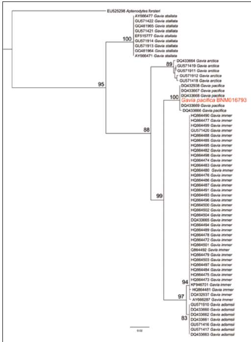
FIGURE 2 Mitochondrial COI gene maximum-likelihood phylogeny of five loon Gavia species, including bird from Silvaplansersee, Graubünden, Switzerland, high-lighted in red, which falls into well-supported clade of Pacific Loon G. pacifica . Node labels indicate bootstrap support for each node in percent.
