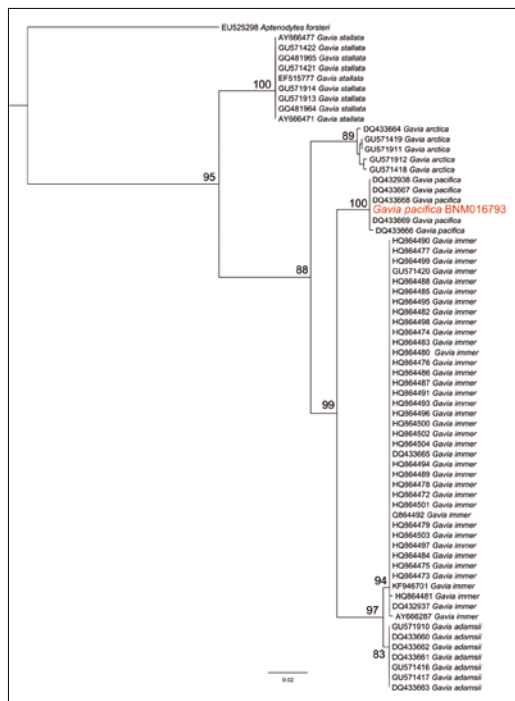
FIGURE 2 Mitochondrial COI gene maximum-likelihood phylogeny of five loon Gavia species, including bird from Silvaplanagersee, Graubünden, Switzerland, high-lighted in red, which falls into well-supported clade of Pacific Loon G. pacifica . Node labels indicate bootstrap support for each node in percent.
