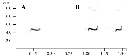
FIGURE 1 Warning calls of Three-banded Plover Charadrius tricoloris , Abu Simbel, Egypt, 1 May 2012 (Wieland Heim). A monosyllabic call, B disyllabic call (made with Avisoft SASLab Pro, Sample rate 24 kHz, FFT-Length 512, Frame 50%, Window Hann, Overlap 87,5%). Sonagram by Karl-Heinz Frommolt.
